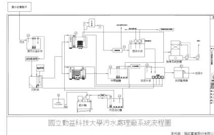
▲ Wastewater Treatment System Flow Diagram
